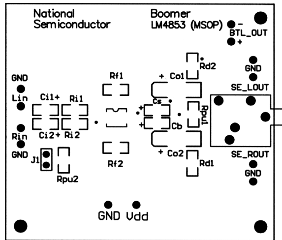
FIGURE 3. Recommended MM PC Board Layout: Component-Side SilkScreen
